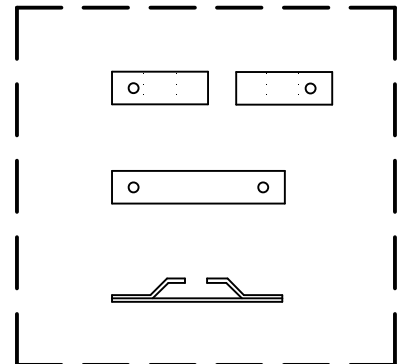
Fairleads – all .01" brass
