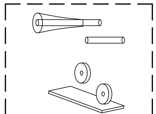
Horn – 1"x1/16 copper wire with filler to make trumpet – solder to 1/4" brass disks and 1"x1/4" brass plate base.
