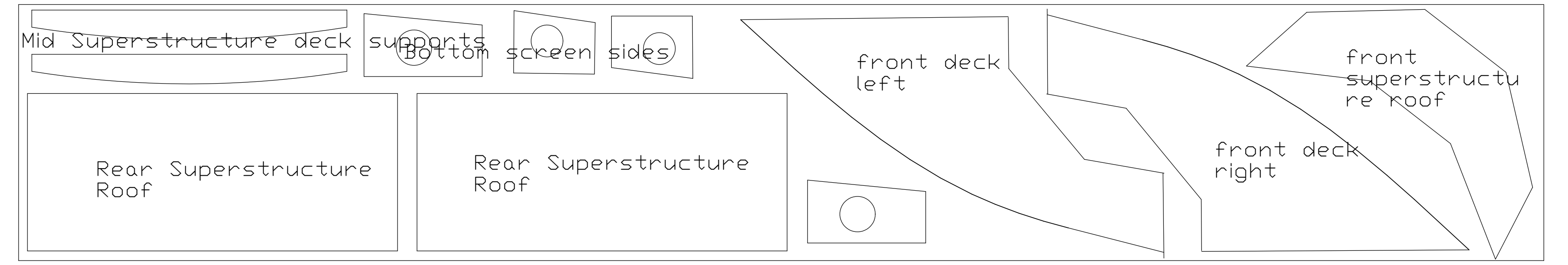
1/16" deck
